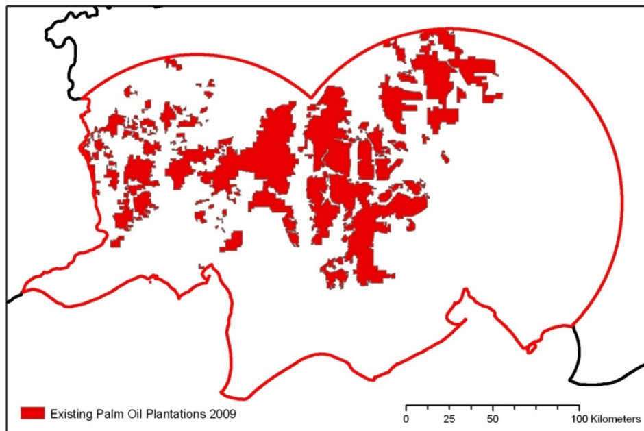
Figure 22. Existing palm oil plantations at project start interpreted and digitized from Landsat 7 ETM+ satellite imagery path-row 118-061 and 118-062 June 7; 119-061 and 199-062 May 13; 120-061 and 120-062 August 8.
