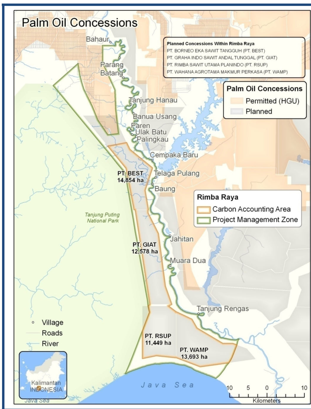
Figure 3. Permitted and Planned Oil Palm Concessions in and around the Project Management Zone. The Carbon Accounting Area is coincident with planned oil palm concessions but excludes the area of active concession and 3km buffer south of the active concession.
