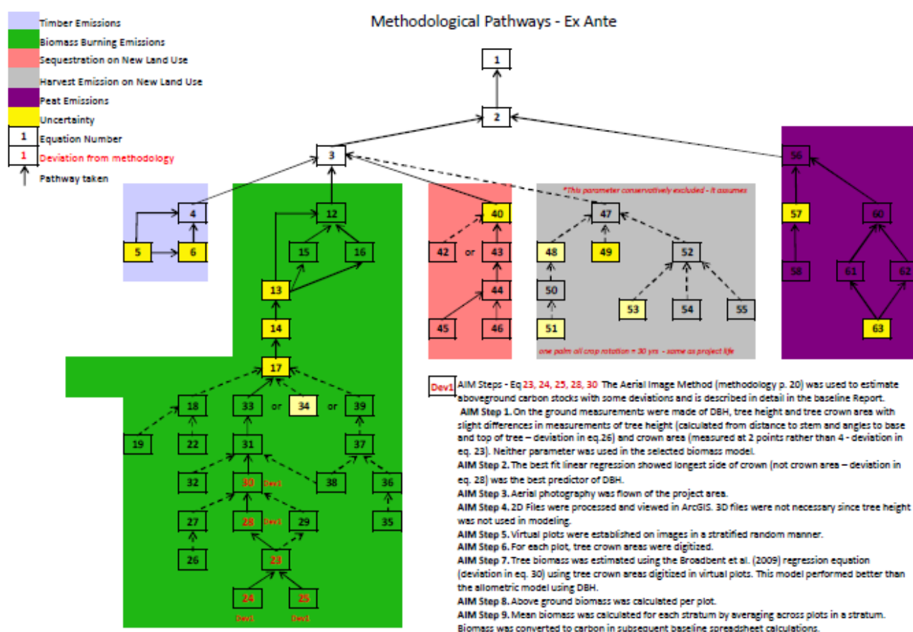
Figure 29. Conceptual diagram of baseline equations and methodological pathways used to calculate Ex-Ante GHG emissions
