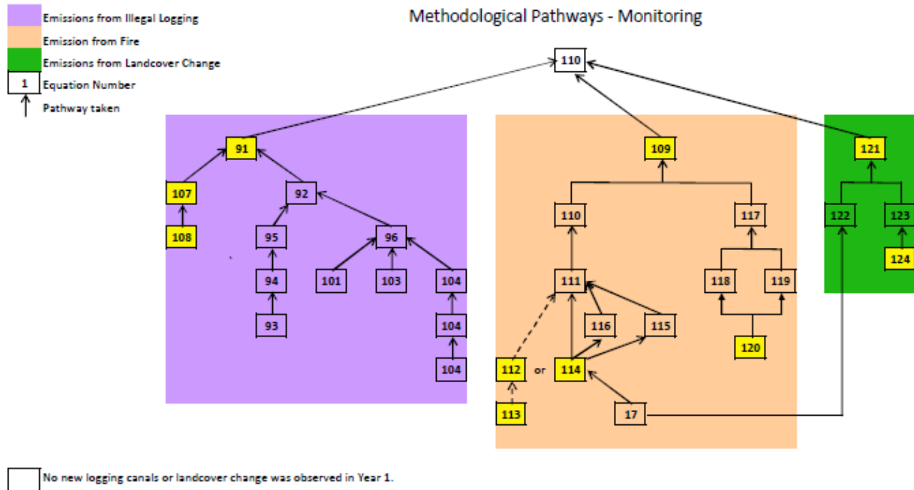
Figure 16. Methodological pathways used to calculate ex post net actual GHG emissions avoided. Pathways included in annual monitoring are shown as solid line arrows. Equations that include at least one parameter for which uncertainty estimation is required are shown in yellow boxes. Note that all pathways are implemented only as required each year. For example, equations 107 and 108, logging emissions associated with peat drainage, were not used in year 1 because there were no new logging canals.
