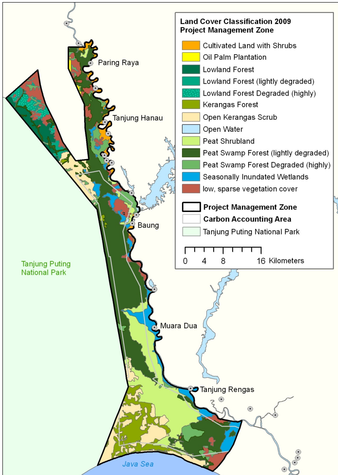
Figure 6. Rimba Raya Vegetation and Land Cover 2009
